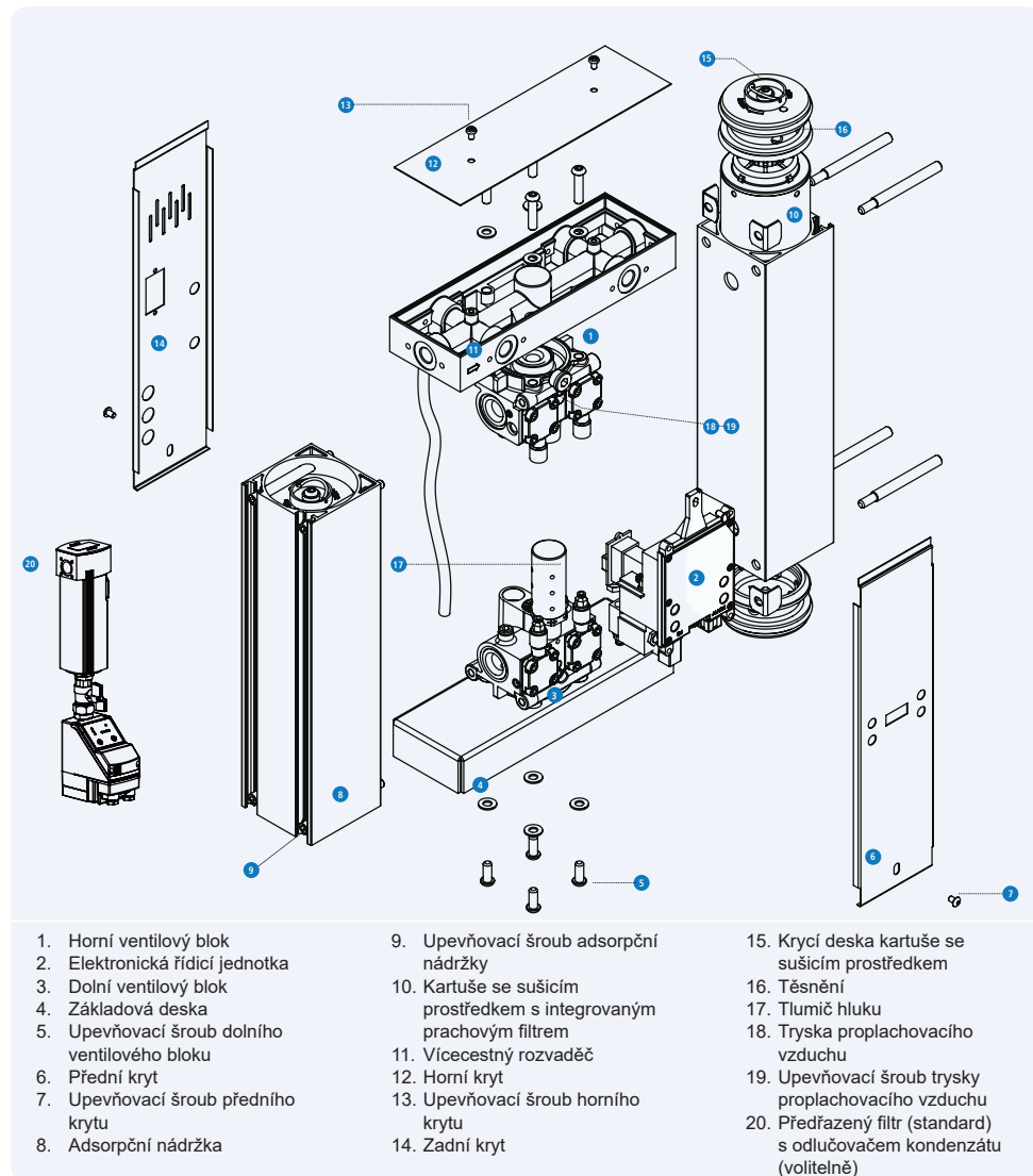
Obr. 10.1: Modely DRYPOINT® AC 171
