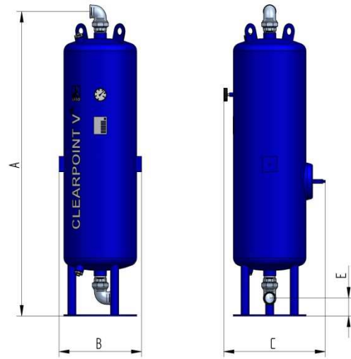
Dimensions CLEARPOINT® L 240 – 295 V
